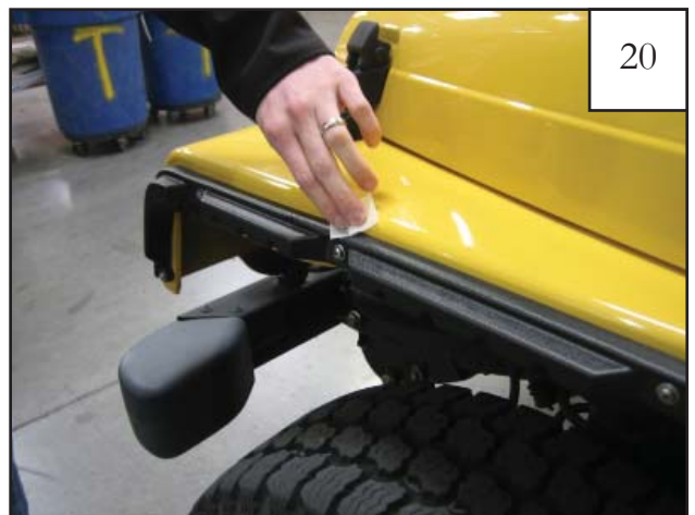
Use one supplied alcohol prep pad to clean the sheet metal above each inner piece in preparation to tape the edge trim to the sheet metal. This must be done for proper flare installation.
