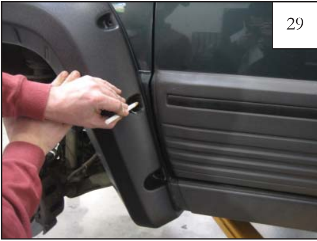
Hold flare in place on vehicle, mark hole locations onto fender through holes drilled in pockets of flare.
