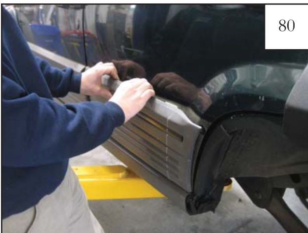
80 Remove the body side cladding from the vehicle. First, lift up by top edge to release top of cladding. Then pull bottom of cladding straight out from side of vehicle.
