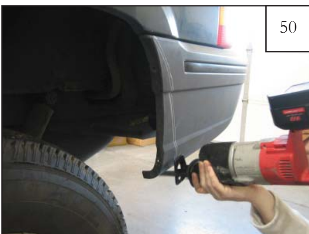
Using the reciprocating saw, cut bumper along offset line. Clean edge with a utility knife.
